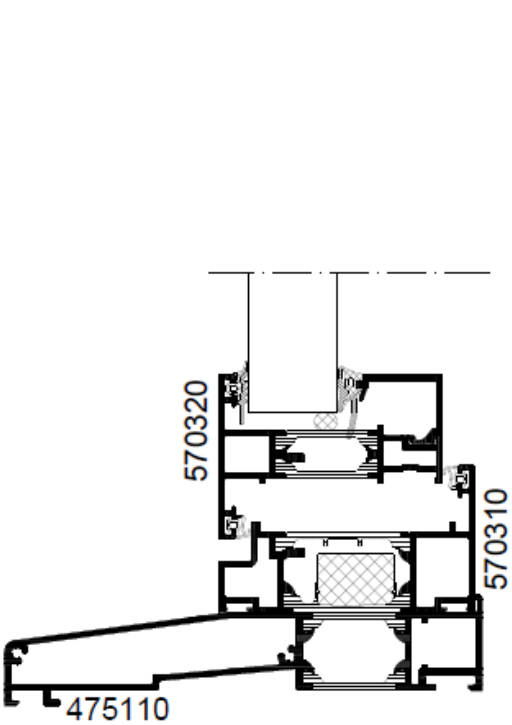
Cill options- 150mm & 180mm
