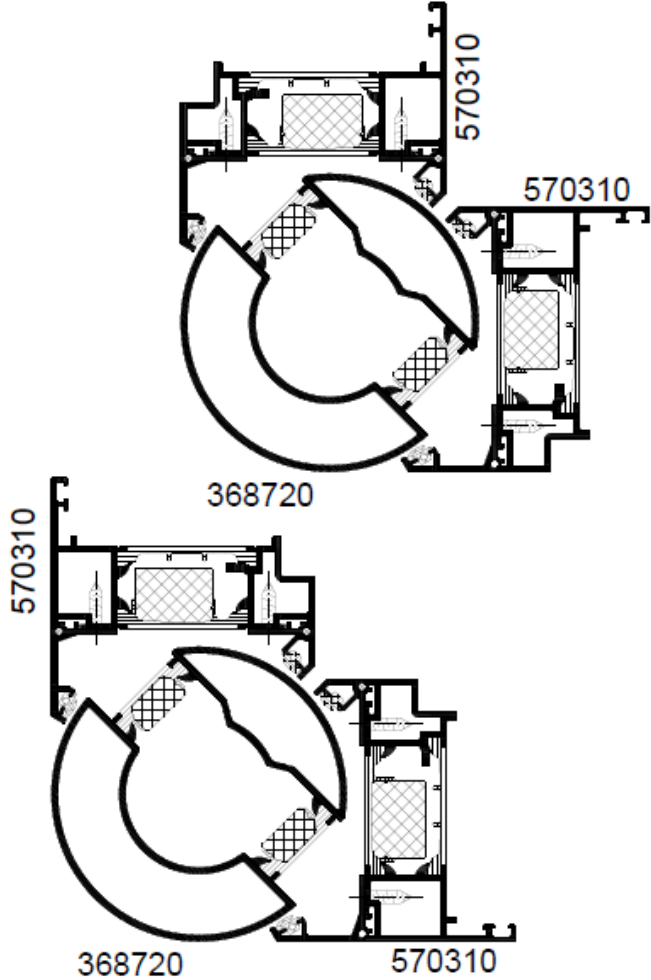
Variable bay pole with option for dual colour
