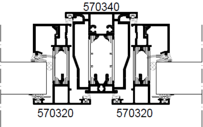
Opening vent transom / mullion with Screwport connection
