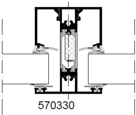
Fixed light transom / mullion with Screwport connection
