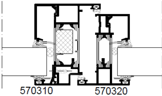
Fixed light next to opening window internally beaded with Z-profile
