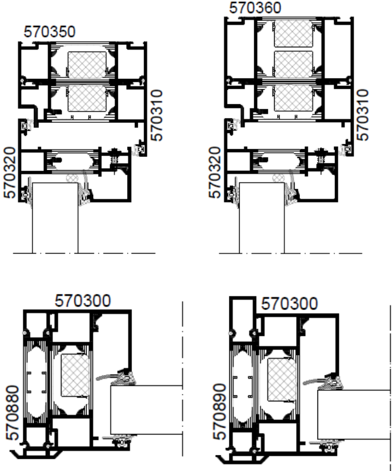
Range of coupling pieces and extension packers
