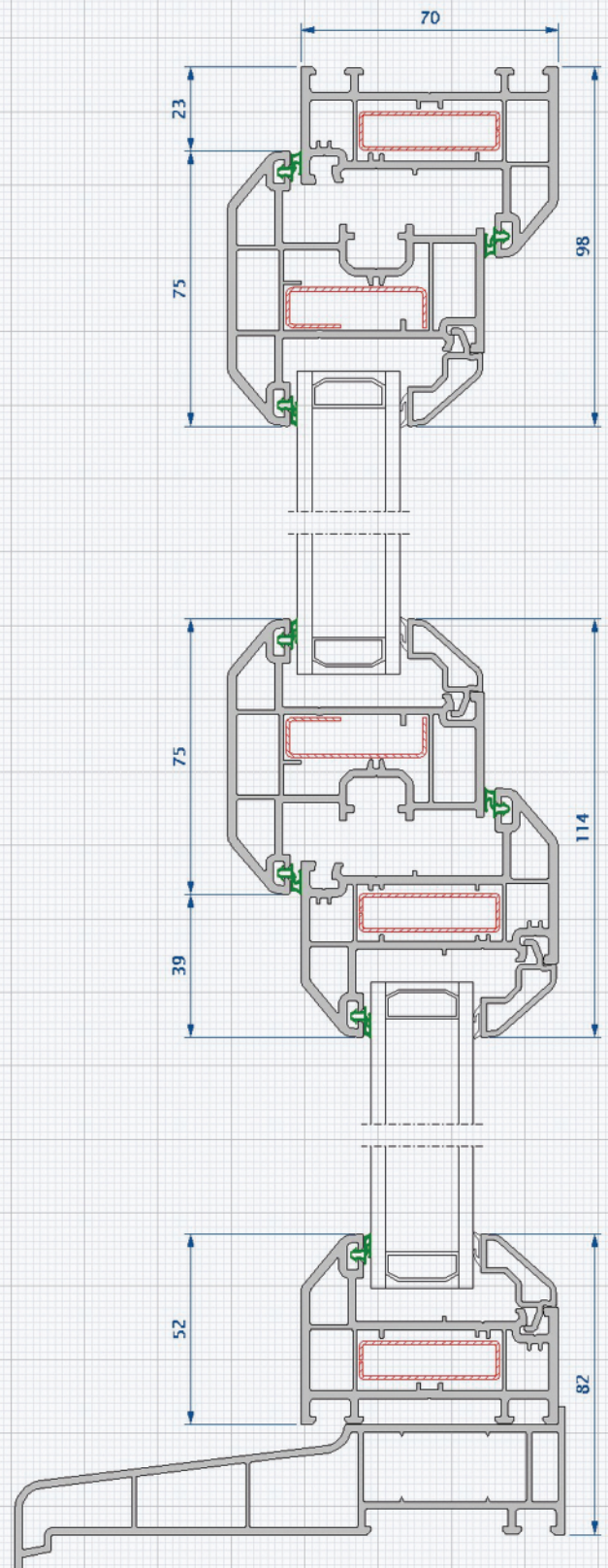
Scale 1:2 2500 chamfered internally glazed casement window profile section
